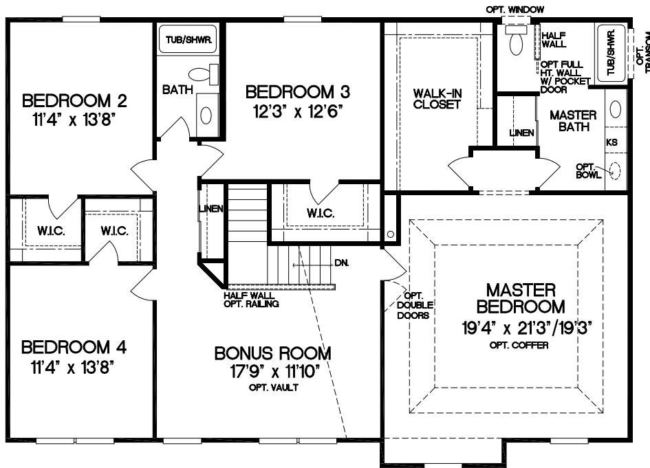
STD. SECOND FLOOR PLAN
